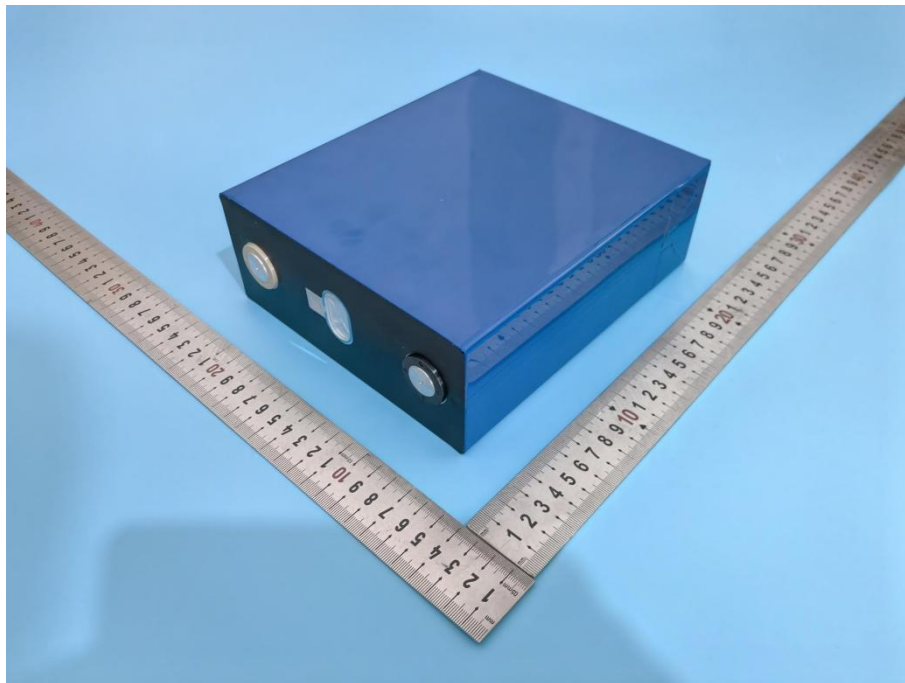
Photo 8 电芯正面 Front view of Cell
